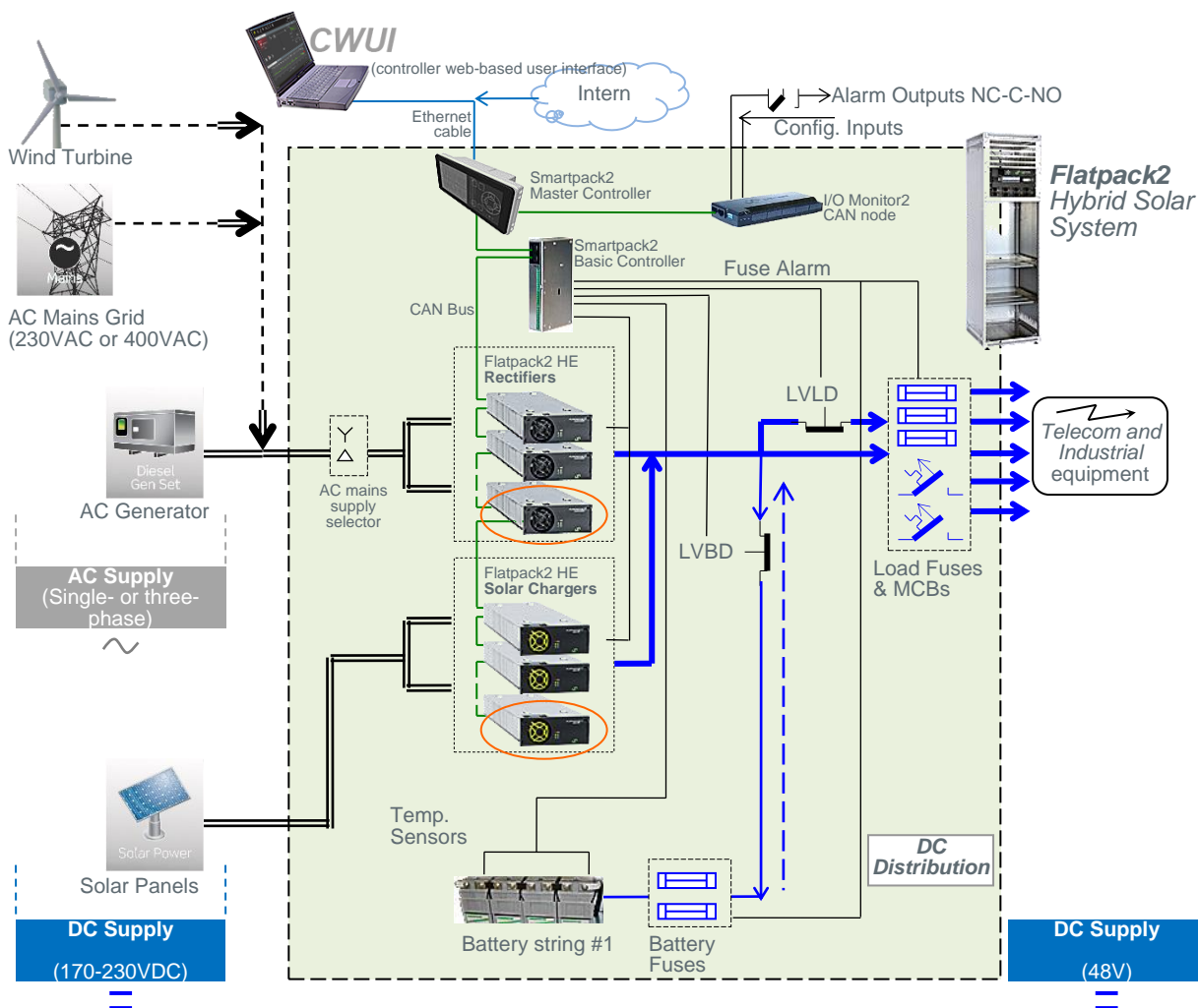
Figure 2 Typical hybrid, solar Flatpack2 PS system for DC power supply of telecom or industrial equipment
